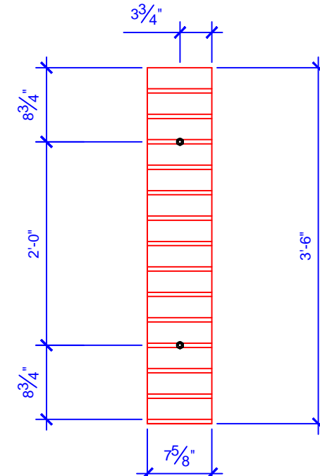
BOLT LAYOUT 8" LINTLE DETAIL 9/A4.14
