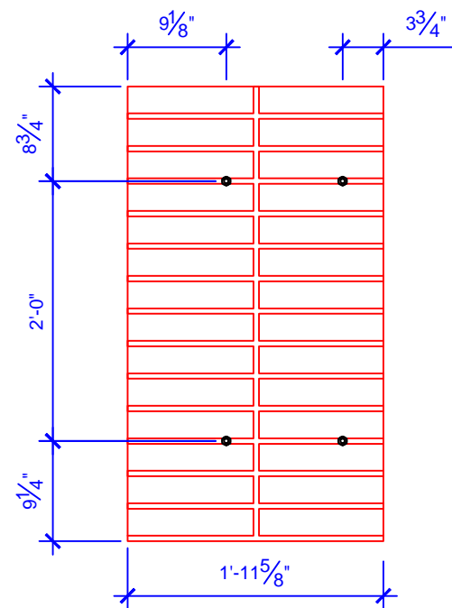
BOLT LAYOUT 24" LINTLE 1/A4.17
