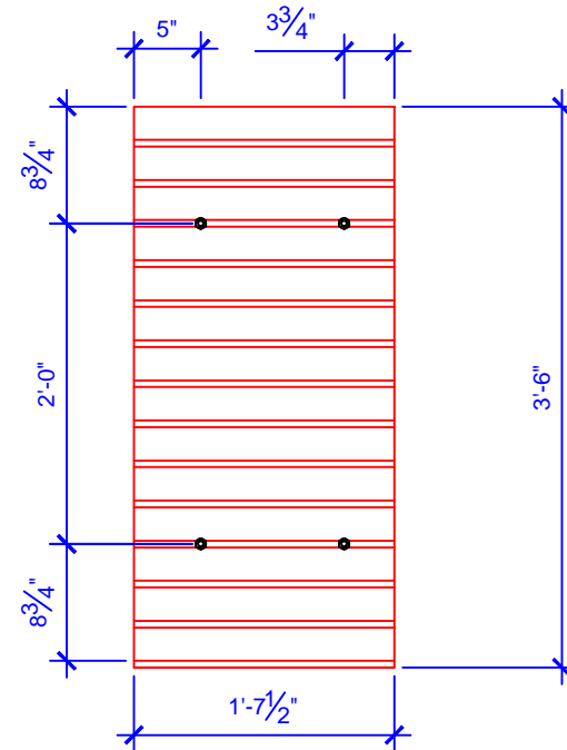
BOLT LAYOUT 20" LINTLE DETAIL 6/A4.14
